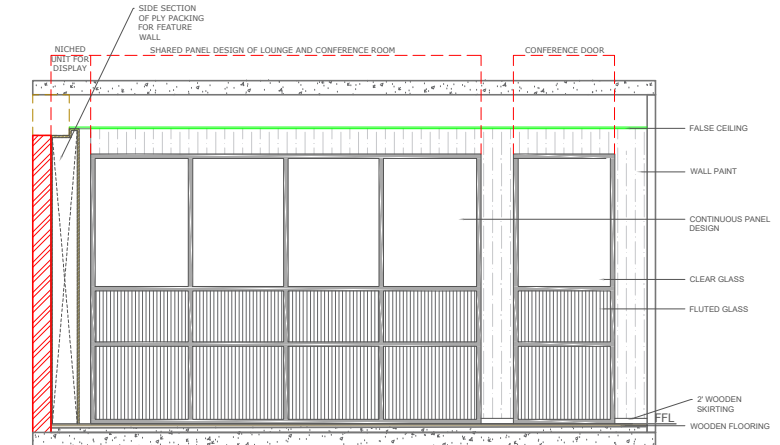
3 SECTION CC'
