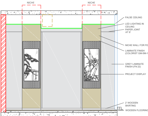
4 SECTION DD'
