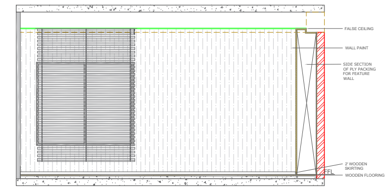
1 SECTION AA'
